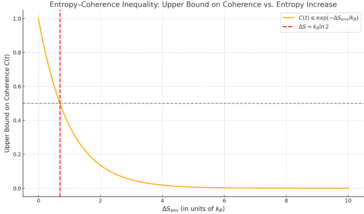
In Figure 5 : The x-axis the entropy generated in the environment \Delta S_{env} (in units of k_B ). The y-axis is the upper bound on coherence C(t) , defined by the trace-norm distance from the fully dephased state. The orange curve plots the primary inequality. The red vertical line indicates the minimum entropy increase associated with a Landauer bit-flip: \Delta S = k_B \ln 2 , below which full classical definiteness may not yet emerge. The gray horizontal line at C(t) = 0.5 marks a mid-coherence benchmark for visual reference (Landauer crossover).
