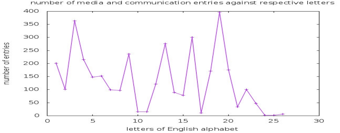
FIG. 4. The vertical axis is the number of entries of the Oxford Dictionary Of Media and Communication, [1], and the horizontal axis is the respective letters. Letters are represented by the sequence number in the alphabet or, dictionary sequence,[1].
