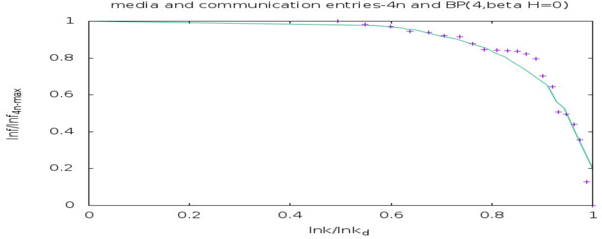
FIG. 9. The vertical axis is \frac{\ln f}{\ln f_{\text{nextnextnextnext-max}}} and the horizontal axis is \frac{\ln k}{\ln k_{\text{lim}}} . The + points represent the entries of the Oxford Dictionary Of Media and Communication, with the fit curve being the Bethe-Peierls curve, BP(4, \beta H = 0 ), with four nearest neighbours, in the absence of external magnetic field.
