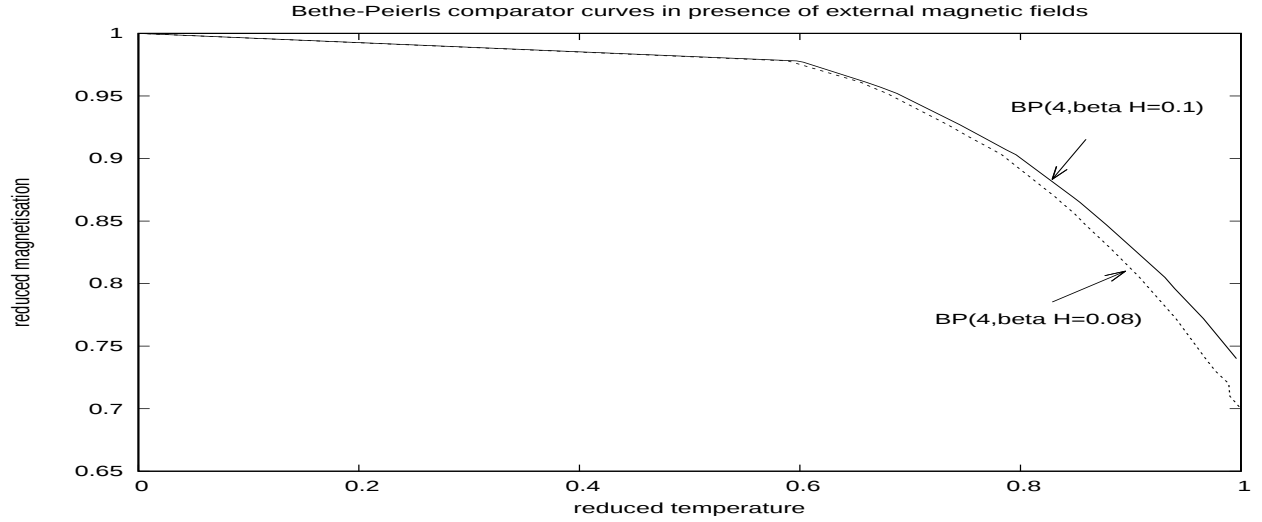
FIG. 3. Reduced magnetisation vs reduced temperature curves for Bethe-Peierls approximation in presence of little external magnetic fields, for four nearest neighbours, with \beta H = 2m .
