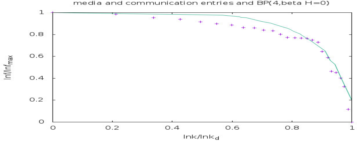
FIG. 5. The vertical axis is \frac{\ln f}{\ln f_{\max}} and the horizontal axis is \frac{\ln k}{\ln k_{\lim}} . The + points represent the entries of the Oxford Dictionary Of Media and Communication, with the fit curve being the Bethe-Peierls curve, BP(4, \beta H = 0 ), with four nearest neighbours, in the absence of external magnetic field.
