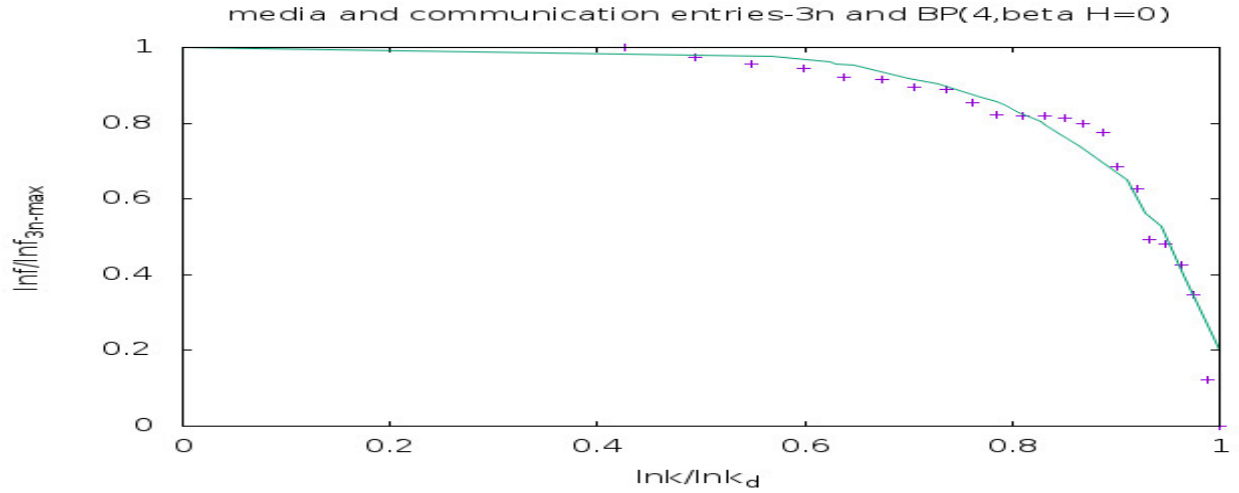
FIG. 8. The vertical axis is \frac{\ln f}{\ln f_{\text{nextnextnext-max}}} and the horizontal axis is \frac{\ln k}{\ln k_{\text{lim}}} . The + points represent the entries of the Oxford Dictionary Of Media and Communication, with the fit curve being the Bethe-Peierls curve, BP(4, \beta H = 0 ), with four nearest neighbours, in the absence of external magnetic field.
