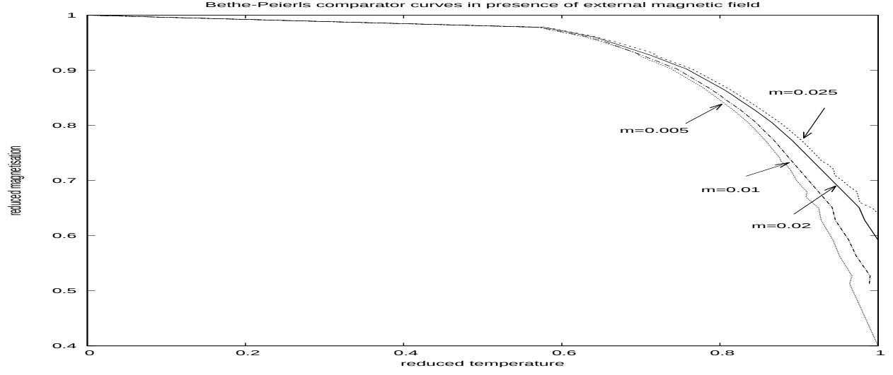
FIG. 2. Reduced magnetisation vs reduced temperature curves for Bethe-Peierls approximation in presence of little external magnetic fields, for four nearest neighbours, with \beta H = 2m .
