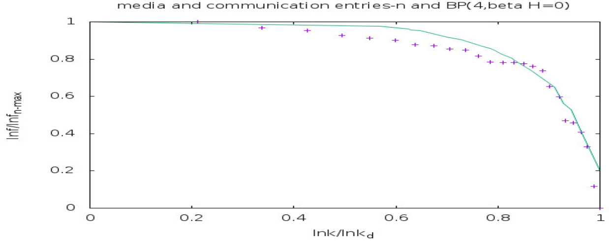
FIG. 6. The vertical axis is \frac{\ln f}{\ln f_{\text{next-max}}} and the horizontal axis is \frac{\ln k}{\ln k_{\lim}} . The + points represent the entries of the Oxford Dictionary Of Media and Communication, with the fit curve being the Bethe-Peierls curve, BP(4, \beta H = 0 ), with four nearest neighbours, in the absence of external magnetic field.
