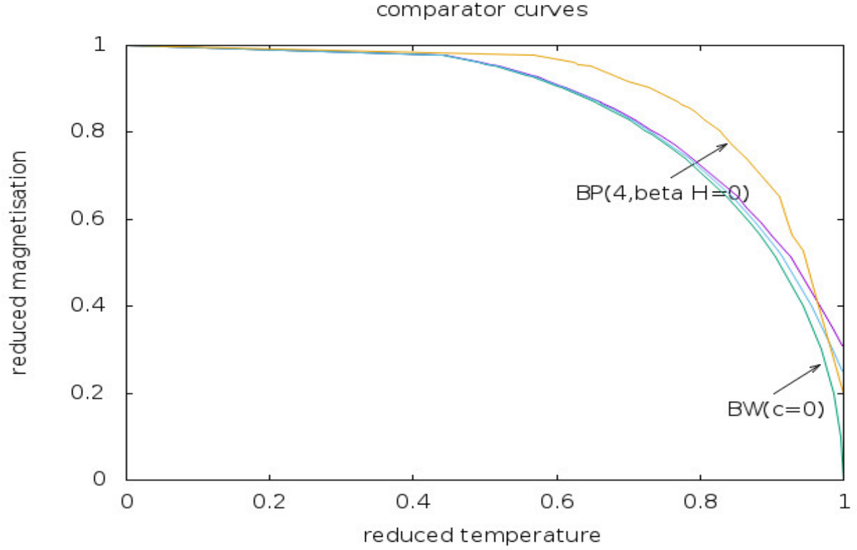
FIG. 1. Reduced magnetisation vs reduced temperature curves, for the Bragg-Williams approximation, in the absence (BW( c=0 )) and in the presence (BW( c=0.005 ), BW( c=0.01 )) of magnetic field, c = 0 , c = \frac{H}{\gamma\epsilon} = 0.005 , c = \frac{H}{\gamma\epsilon} = 0.01 , outwards; and in the Bethe-Peierls approximation, BP(4, \beta H=0 ), in the absence of magnetic field, for four nearest neighbours (outer in the top).
