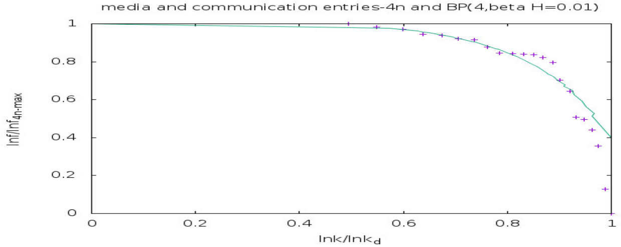
FIG. 10. The vertical axis is \frac{\ln f}{\ln f_{\text{nextnextnextnext-max}}} and the horizontal axis is \frac{\ln k}{\ln k_{\text{lim}}} . The + points represent the entries of the Oxford Dictionary Of Media and Communication, with the fit curve being the Bethe-Peierls curve, BP(4, \beta H = 0.01 ), with four nearest neighbours, in the presence of little external magnetic field.
