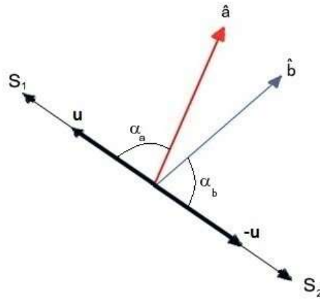
Figure 1: Original positions of the spins and the polarizers axis.
