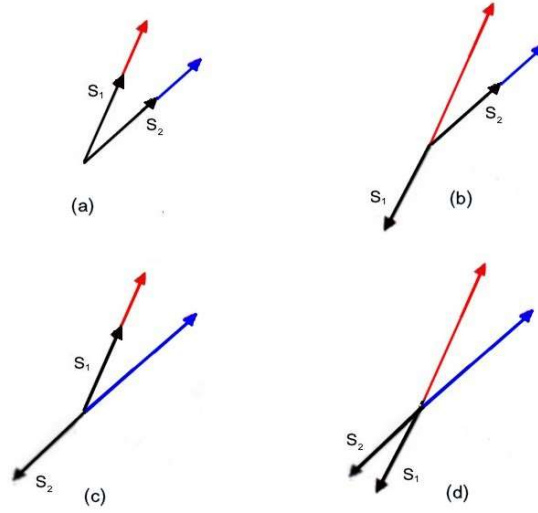
Figure 2: The four possible arrangements of the spins with respect to the polarizer's axis after interaction with the field.
