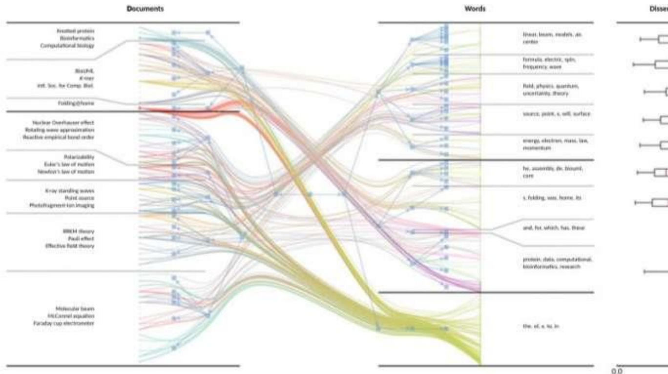
Fig. 5. Inference of hSBM to articles from the Wikipedia. Articles from three categories (chemical physics, experimental physics, and computational biology) are analyzed. The hierarchical level reflects bipartite nature of the network with document nodes (left) and word nodes (right). The grouping on the second hierarchical level is in accordance with the categories. We show examples for nodes that belong to each group on the third hierarchical level (indicated by dotted lines): For word nodes, we show the five most frequent words; for document nodes, we show three (or fewer) randomly selected articles. For each word, we calculate the dissemination coefficient U_D , which quantifies how the word is distributed among documents ( U_D = 1 indicates the expected dissemination from a random null model; the smaller U_D ( 0 < U_D < 1 ), the more unevenly the word is distributed). We show the 5th, 25th, 50th, 75th, and 95th percentile for each group of word nodes on the third level of the hierarchy. Intl. Soc. for Comp. Biol., Intl. Soc. for Comp. Biol., Intl. Soc. for Comp. Biol., Intl. Soc. for Comp. Biol., Intl. Soc. for Comp. Biol.
