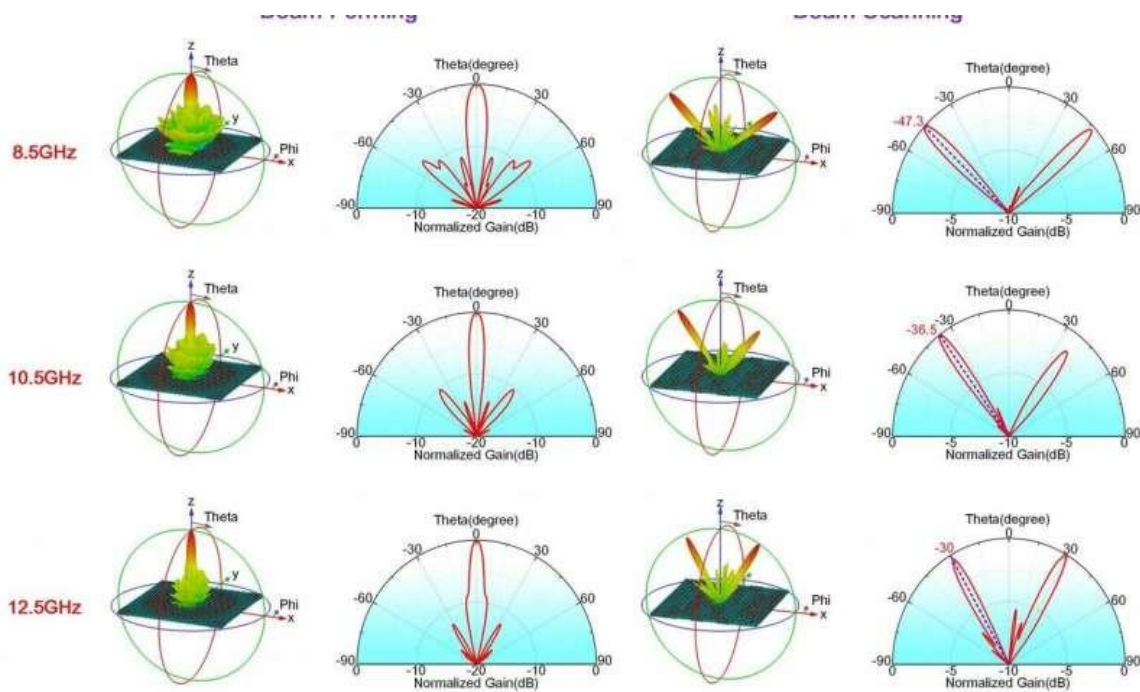
Beam-forming and beam-scanning functionalities of the proposed broadband 1-bit coding metasurface. Credit: Science China Press
