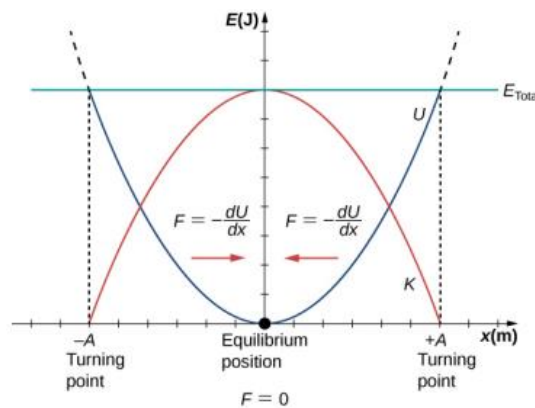
Figure 5: Kinetic (K) and potential energy (U) of an oscillator 47
