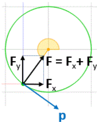
Figure 3: The Zitterbewegung model of an electron
