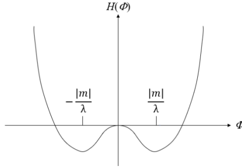
Figure 6. Two local minimums in the Higgs potential of the scalar field \Phi .
