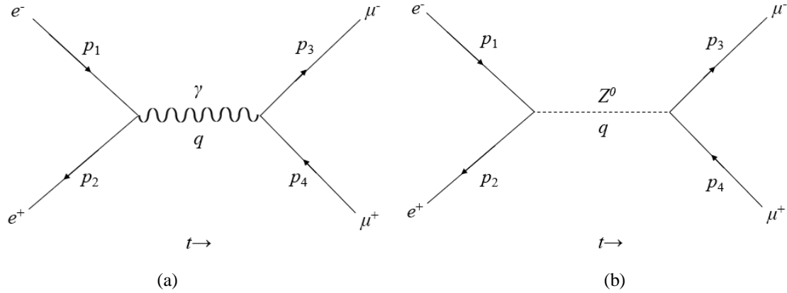
Figure 3. (a) The Feynman diagram about the electromagnetic contribution to e^+ + e^- \rightarrow \mu^+ + \mu^- . (b) The Feynman diagram about the weak contribution to e^+ + e^- \rightarrow \mu^+ + \mu^- .
