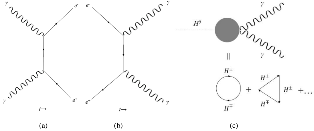
Figure 1. (a) The electron-positron pair production describing in QED. (b) Two-photon production by the electron-positron pair annihilation also describing in QED. The other diagram can be drawn by interchanging two outgoing photons. (c) The neutral Higgs boson decays to two photons including the parts of vertices [8,9].
