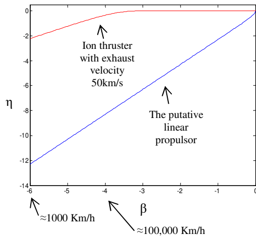
Figure 4 – Log-Log plot of Fraction, η of rest-mass used vs. Fraction of light-speed, β obtained
