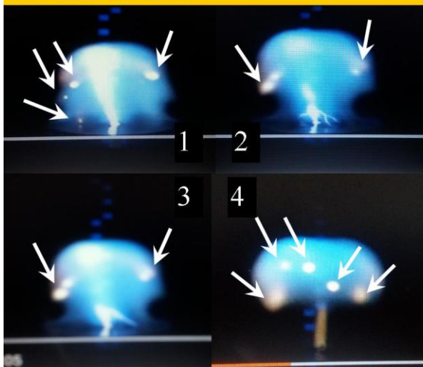
Figure 7, Microscopic Black Holes on Earth.
