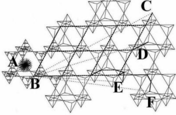
Photon trajectories through the tetrahedral Chiral vacuum lattice.
