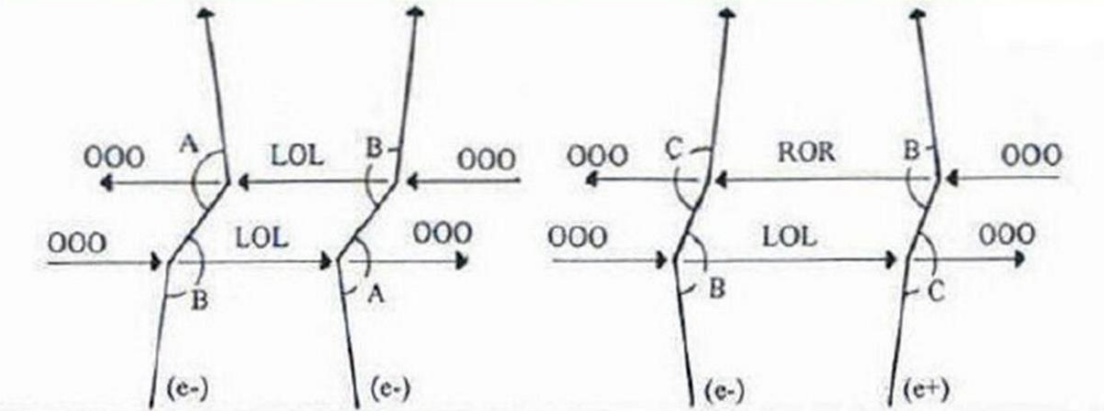
( Above) Alternative Feynman diagrams for electron-positron attraction and electron-electron repulsion by Dipole Repeller system.
