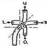
( Above) Alternative Feynman diagrams for electron-positron attraction and electron-electron repulsion by Dipole Repeller system.
