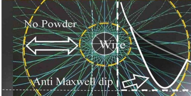
According to Quantum FFF theory, all magnetic fields can be presented as DUAL Magnetic Monopole Photon Vector Arrays. These monopole arrays undergo curvature. As a result, the magnetic field intensity around the Earth and a wire is NOT dropping off with the square of the distance from the source!! The field become stronger polarized away from the source (See images). Close to the current transporting wire the magnetic field strength is zero due to the parallel trajectories of North and South Photons before curvature and polarisation of iron powder (Author: Leo Vuyk)
