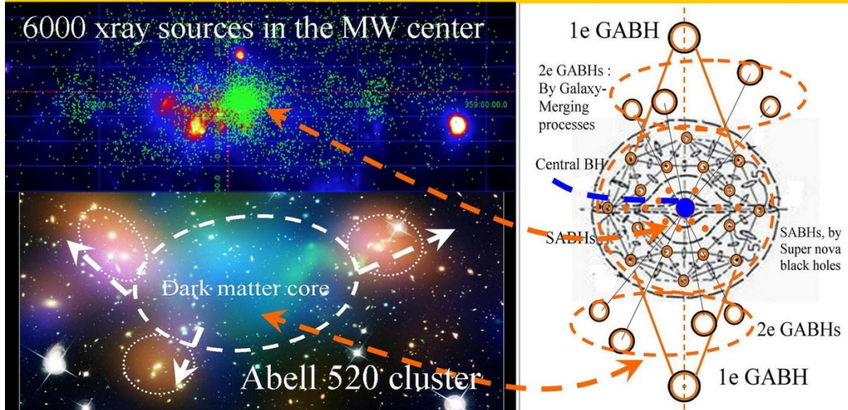
Figure 6, Merger dynamics of NON inertial Dark Matter black holes left behind after merging in the middle.
