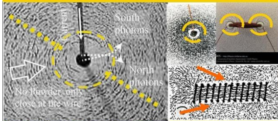
According to Quantum FFF theory, all magnetic fields can be presented as DUAL Magnetic Monopole Photon Vector Arrays. These monopole arrays undergo curvature. As a result, the magnetic field intensity around the Earth and a wire is NOT dropping off with the square of the distance from the source!! The field become stronger polarized away from the source (See images). Close to the current transporting wire the magnetic field strength is zero due to the parallel trajectories of North and South Photons before curvature and polarisation of iron powder (Author: Leo Vuyk)
