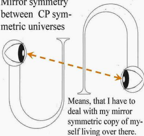
Figure 3, wavefunction collapse between CP symmetric mirror particles by instant entanglement between multi universal bubbles located around the Big Bang central void.
