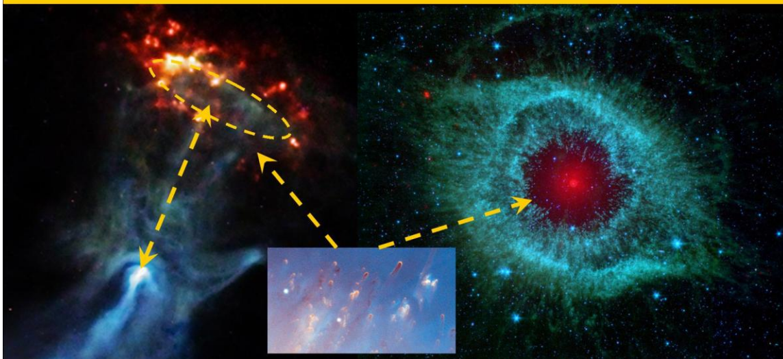
Figure 11, The A-symmetric B 1509-58 nebula , and symmetric Helix nebula as examples of the difference between Fermion and Black hole Quantum Gravity effects.
