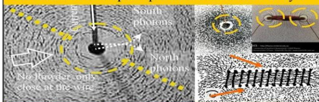
According to Quantum FFF theory, all magnetic fields can be presented as DUAL Magnetic Monopole Photon Vector Arrays. These monopole arrays undergo curvature. As a result, the magnetic field intensity around the Earth and a wire is NOT dropping off with the square of the distance from the source!! The field become stronger polarized away from the source (See images). Close to the current transporting wire the magnetic field strength is zero due to the parallel trajectories of North and South Photons before curvature and polarisation of iron powder (Author: Leo Vuyk)
