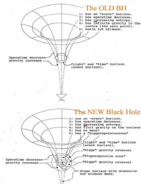
Figure 31, The new black hole
