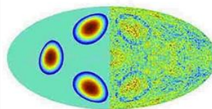
Figure 3, wavefunction collapse between CP symmetric mirror particles by instant entanglement between multi universal bubbles located around the Big Bang central void.
