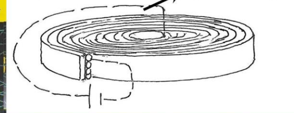
According to Quantum FFF theory, all magnetic fields can be presented as DUAL Magnetic Monopole Photon Vector Arrays. These monopole arrays undergo curvature. As a result, the magnetic field intensity around the Earth and a wire is NOT dropping off with the square of the distance from the source!! The field become stronger polarized away from the source (See images). Close to the current transporting wire the magnetic field strength is zero due to the parallel trajectories of North and South Photons before curvature and polarisation of iron powder (Author: Leo Vuyk)
