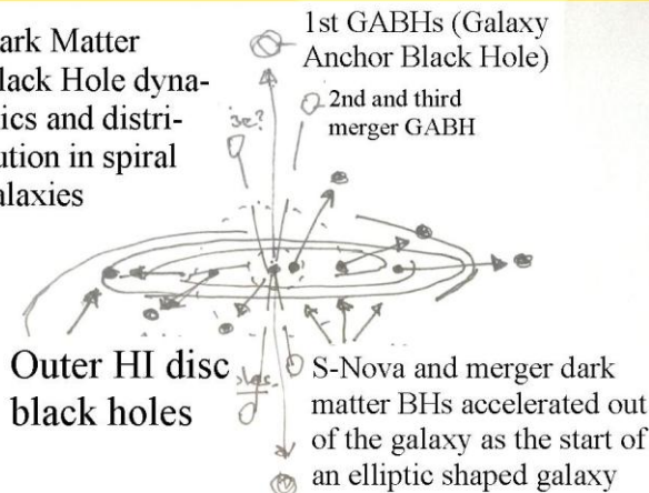
Figure 30, . Dark Matter Black Hole dynamics in spiral galaxies.
