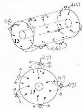
Figure 17, BBBH , the Big Bang Black Hole splintering into smaller BHs and evaporating into the oscillating Axion Higgs Vacuum lattice .
