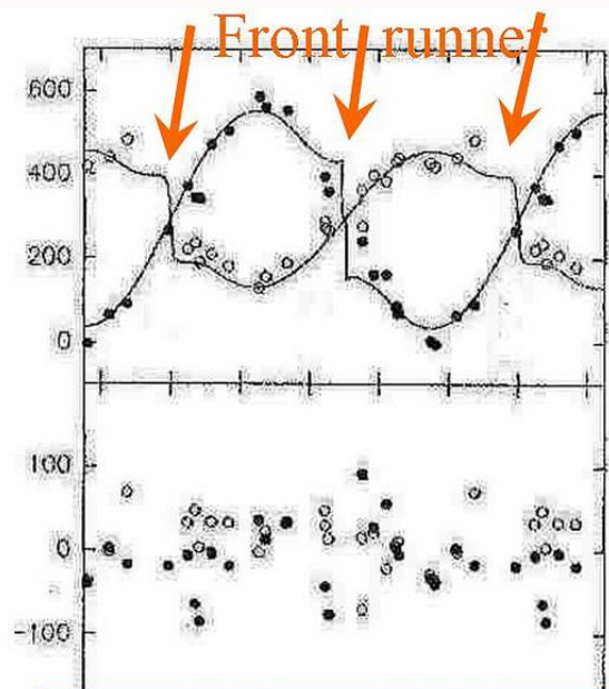
Radial velocity curves for HV2543 binary
