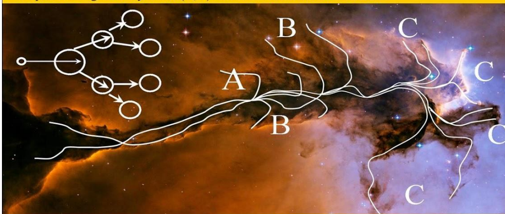
Figure 12, LIGO BH ratios and the BH multiplier splitting process in the Spire- Eagle nebula.
