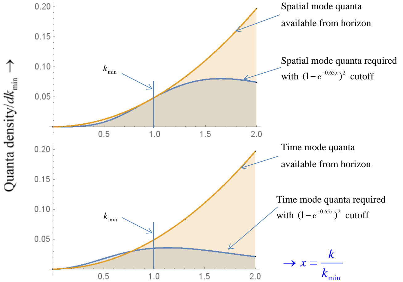
Figure 5.3. 1 plots Eq's.(5.3. 2) & (5.3. 11) as a function of x = k / k_{min} . Going through similar procedures for the time mode quanta as for space modes, we have plotted both time and space. The exponential e^{-0.65x} cutoff fits available and required reasonably for k < k_{min} in both cases; also showing there should be an adequate supply of time mode quanta from the horizon for all infinitesimal mass particles. The spatial mode crosses @ k = k_{min} . Both plots always look the same at all cosmic times T . And, in any metric only the value of k_{min} changes. It only works in an expanding flat universe. Equating required and available spatial modes @ k = k_{min}
