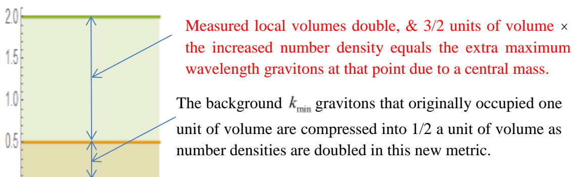
Figure 5.2. 2 An infinitesimal local volume in a metric where \sqrt{g_{rr}} = \gamma_M = 2 .
