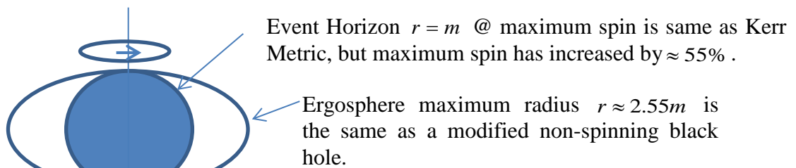
Figure 8.1. 1 Modified Kerr Metric with the dimensionless parameter A changed from
