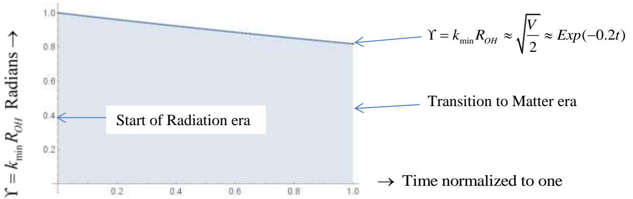
Figure 5.3. 2 The Radiation dominant era where \Upsilon = k_{\min} R_{OH} starts at \approx 1
