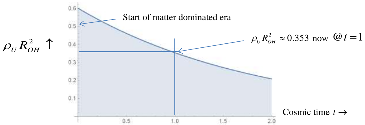
Figure 5.3. 7 plots \rho_U R_{OH}^2 \approx 0.6 \text{Exp}(-0.53t) in Planck units to twice the universe age.
