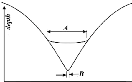
Figure 3. What if mass was constant?
