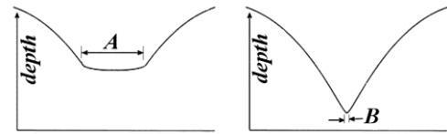
Figure 1. Depression of spacetime depth by mass
