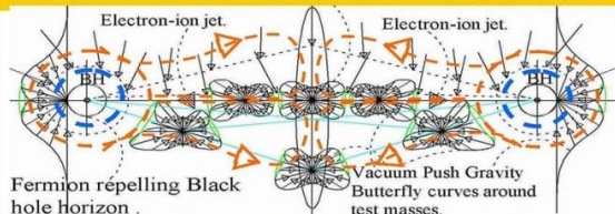
Figure 19, Even the sun seems to have polar dual black hole Herbig Haro remnants and is able to produce and expel gas planets (failed stars) at this age.
