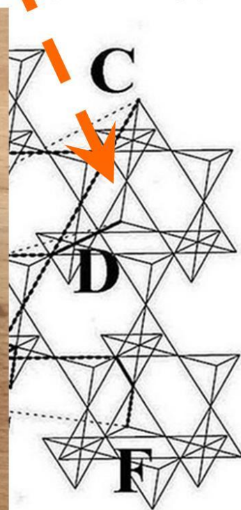
Figure 5, A stable black hole nucleus is large enough to “eat” the vacuum particles and grow by it.
