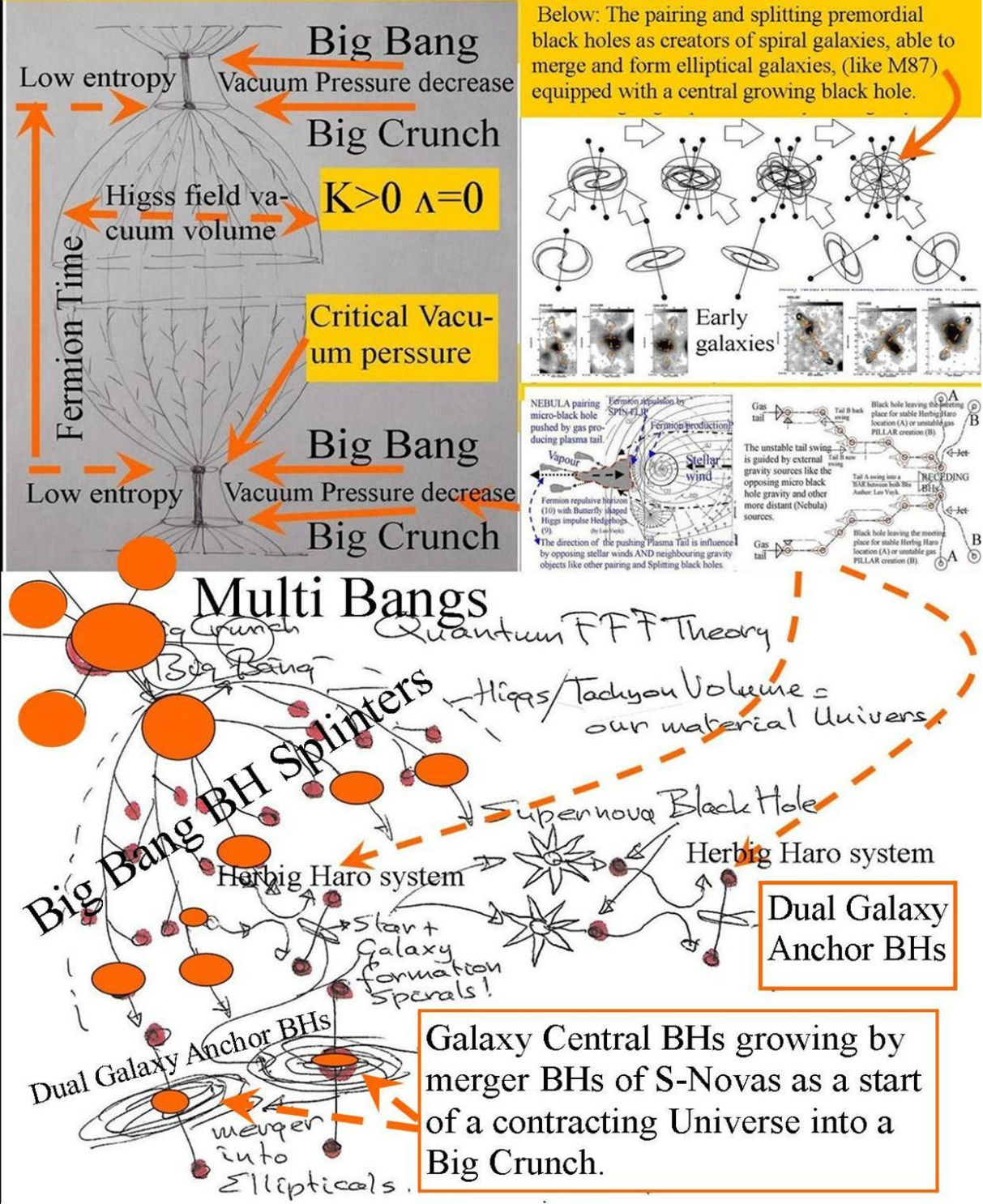
Figure 14, The Cyclic Multiverse.
