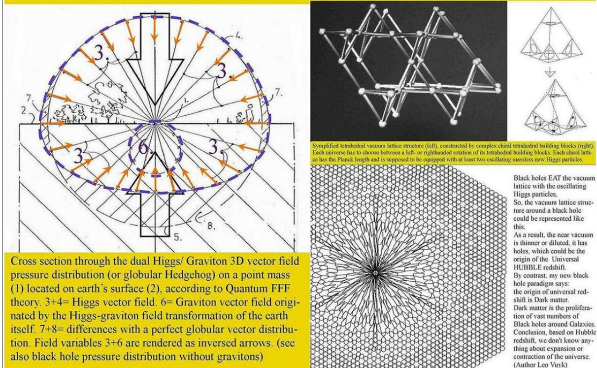
Figure 24, Quantum dipole repeller gravity ( the oscillating Casimir vacuum ) combined with less pressure from pushing gravitons.
