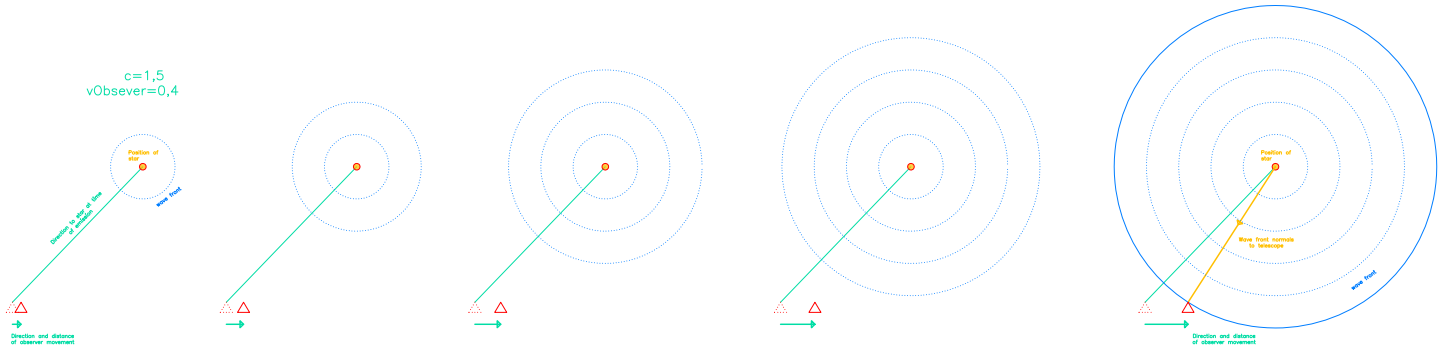
Fig. 11: Light propagation from source with 0,3 seconds steps, earth's speed 0,4 \text{ km/s}
