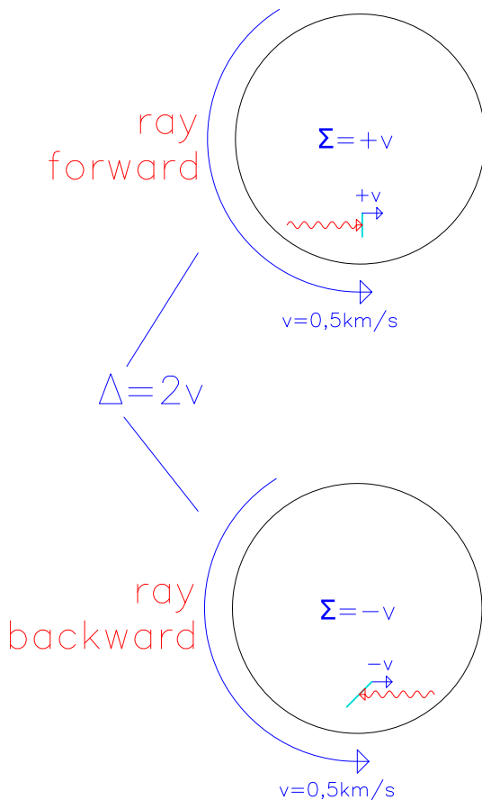
Fig. 3: Relevant velocities on Michelson/Morley experiment in fully entrained ether
