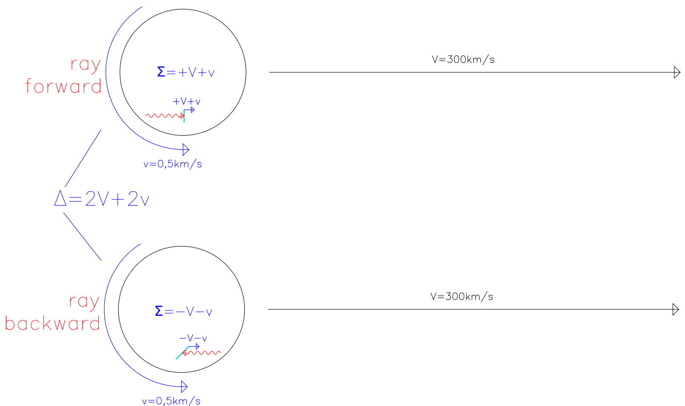
Fig. 2: Relevant velocities on Michelson/Morley experiment in static ether
