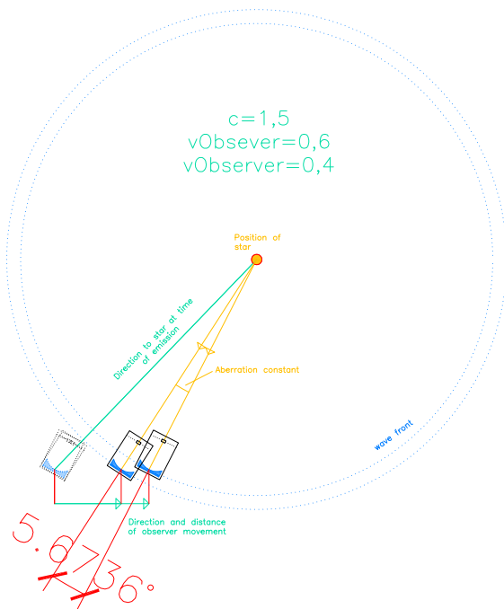
Fig. 12: Overlay both situations 0,6 and 0,4 \text{ km/s}
