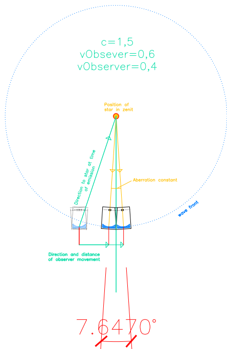
Fig. 13: Overlay 0,6 and 0,4 km/s but on 90^\circ middling observation angle
