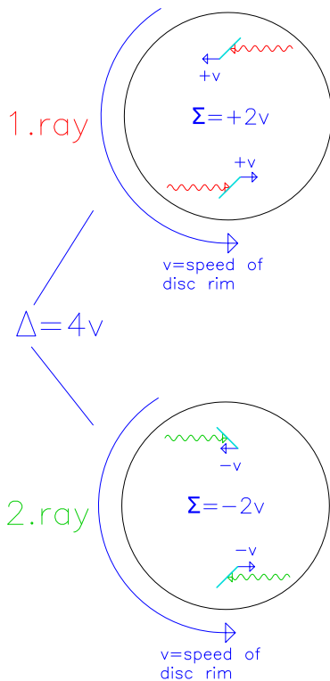
Fig. 6: Relevant velocities on Sagnac experiment in fully entrained ether
