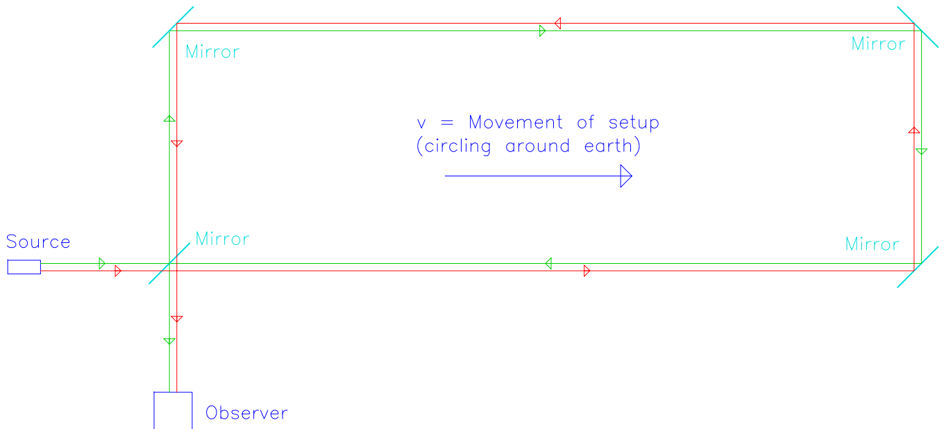
Fig. 7: Schematic setup of the Michelson/Gale/Pearson experiment
