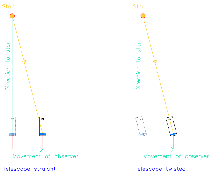
Fig. 8: Stellar aberration by classic explanation
