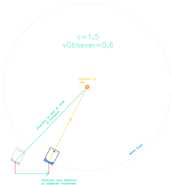
Fig. 10 Telescope directed to source.
