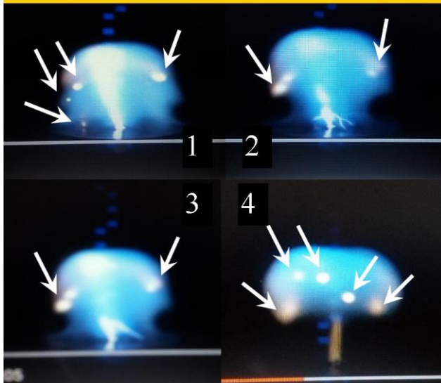
Figure 00, Microscopic Black Holes on Earth.
