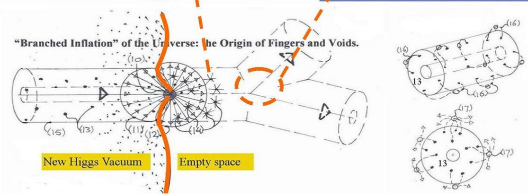
Figure 10 , BBBH , the Big Bang Black Hole splintering into smaller BHs and evaporating into the oscillating Axion Higgs Vacuum lattice .
