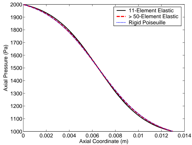
Figure 4. Axial pressure as a function of axial coordinate for a converging-diverging elastic tube with parabolic geometry having L = 0.013 m, R_{min} = 0.0017 m, R_{max} = 0.0025 m, and \beta = 28059.0 Pa.m. The fluid properties are: \rho = 1100 kg.m -3 and \mu = 0.006 Pa.s while the inlet and outlet pressures are: p_i = 2000 Pa and p_o = 1000 Pa. The Poiseuille-type flow uses a rigid tube with the same unstressed geometry and the same \mu and boundary pressures. The converged flow rate for the elastic Navier-Stokes and rigid Poiseuille-type flows are respectively: Q_e = 6.58209 \times 10^{-5} m 3 .s -1 and Q_r = 6.62929 \times 10^{-5} m 3 .s -1 while the analytic flow rate for the rigid tube as obtained from the second equation in Table 2 is Q_a = 6.62051 \times 10^{-5} m 3 .s -1 .
