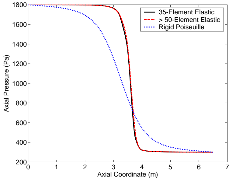
Figure 7. Axial pressure as a function of axial coordinate for a converging-diverging elastic tube with sinusoidal geometry having L = 6.5 m, R_{min} = 0.2 m, R_{max} = 0.5 m, \beta = 5064.2 Pa.m. The fluid properties are: \rho = 900 kg.m -3 and \mu = 0.06 Pa.s while the inlet and outlet pressures are: p_i = 1800 Pa and p_o = 300 Pa. The Poiseuille-type flow uses a rigid tube with the same unstressed geometry and the same \mu and boundary pressures. The converged flow rate for the elastic Navier-Stokes and rigid Poiseuille-type flows are respectively: Q_e = 0.396769 m 3 .s -1 and Q_r = 8.74955 m 3 .s -1 while the analytic flow rate for the rigid tube as obtained from the fifth equation in Table 2 is Q_a = 8.73370 m 3 .s -1 .
