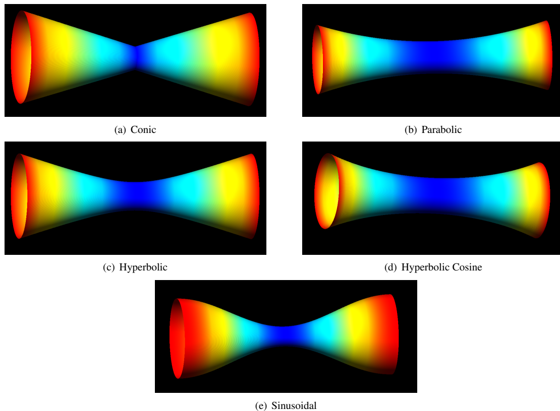
Figure 1. Converging-Diverging tube geometries used in the current investigation.
