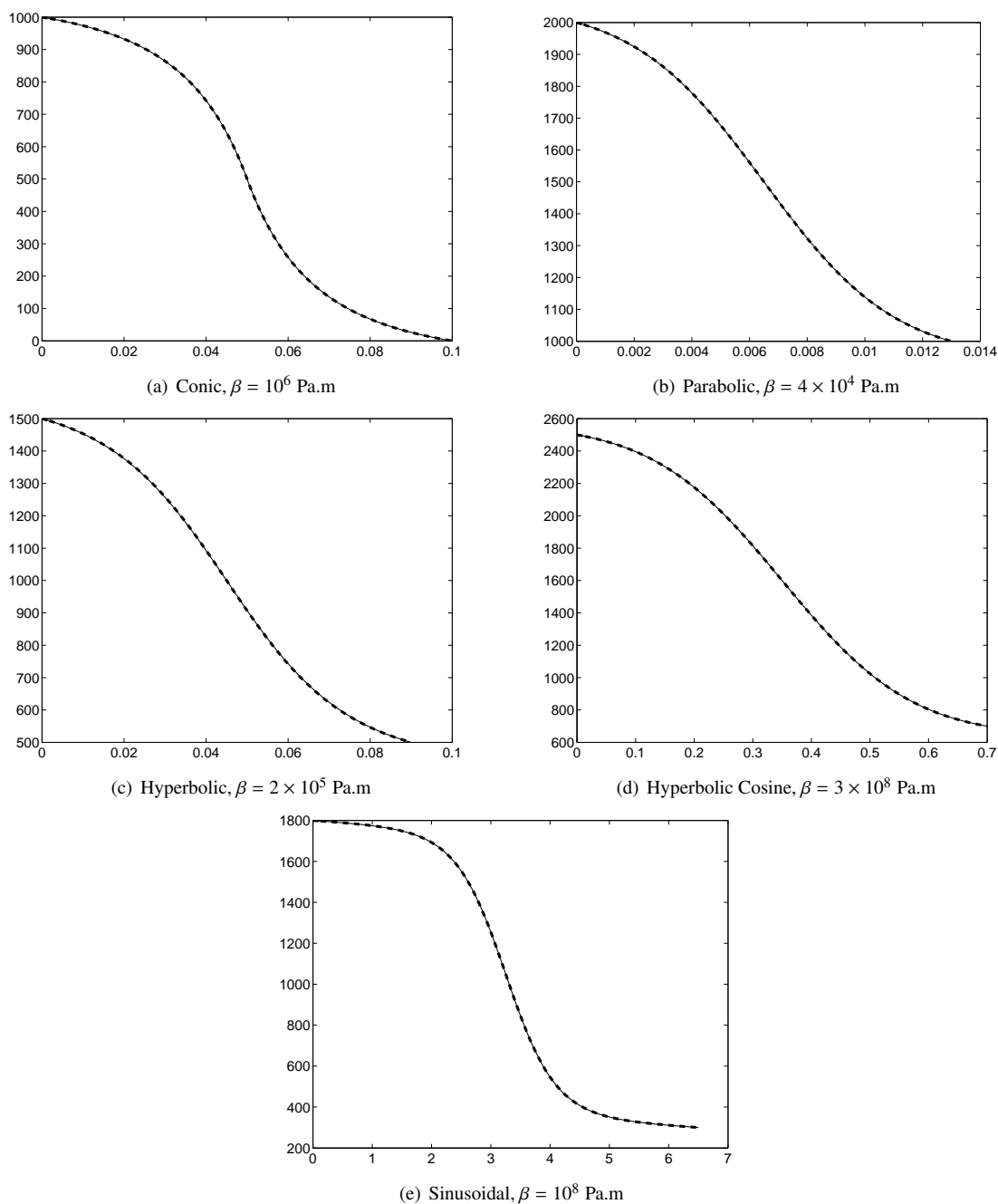
Figure 8. Comparing the converged Poiseuille-type rigid tube flow (solid) to the converged elastic tube flow with high wall stiffness of the given \beta (dashed) for the five examples of Figures 3-7. In all the five sub-figures, the vertical axis represents the axial pressure in pascals while the horizontal axis represents the tube axial coordinate in meters. The converged numeric flow rate in each case for the rigid and elastic models is virtually identical to the corresponding Poiseuille-type analytic flow rate given in Figures 3-7.
