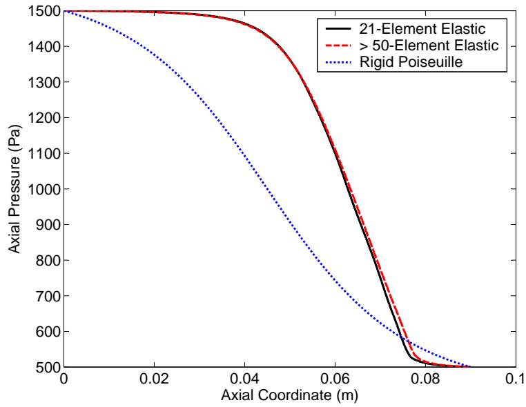
Figure 5. Axial pressure as a function of axial coordinate for a converging-diverging elastic tube with hyperbolic geometry having L = 0.09 m, R_{min} = 0.004 m, R_{max} = 0.006 m, and \beta = 23.6 Pa.m. The fluid properties are: \rho = 800 kg.m -3 and \mu = 0.002 Pa.s while the inlet and outlet pressures are: p_i = 1500 Pa and p_o = 500 Pa. The Poiseuille-type flow uses a rigid tube with the same unstressed geometry and the same \mu and boundary pressures. The converged flow rate for the elastic Navier-Stokes and rigid Poiseuille-type flows are respectively: Q_e = 0.000147335 m 3 .s -1 and Q_r = 0.000934645 m 3 .s -1 while the analytic flow rate for the rigid tube as obtained from the third equation in Table 2 is Q_a = 0.000933394 m 3 .s -1 .
