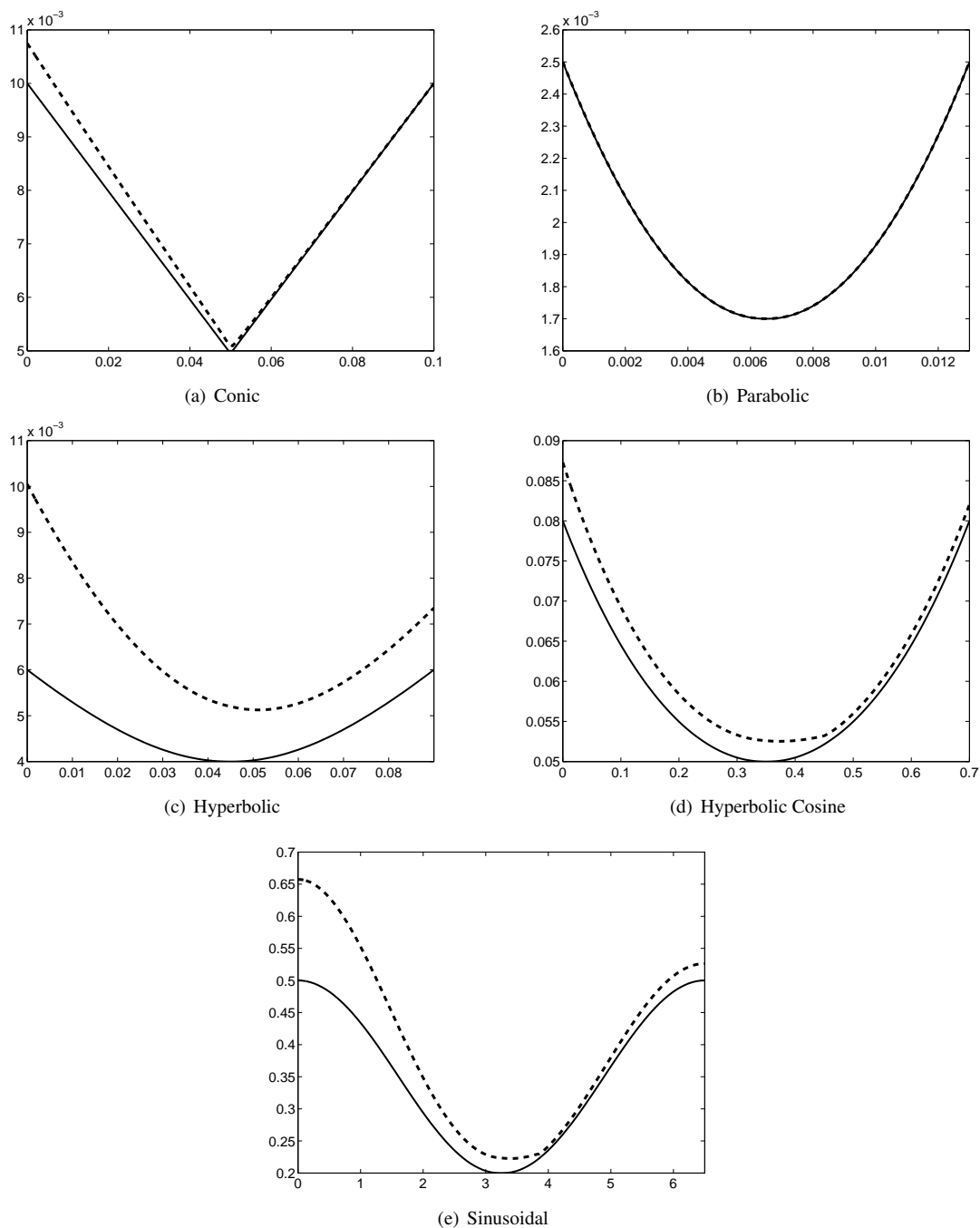
Figure 9. Comparing the elastic tube unstressed radius (solid) to the stressed radius (dashed) as a function of the tube axial coordinate for the five examples of Figures 3-7. In all the five sub-figures, the vertical axis represents the tube radius in meters and the horizontal axis represents the tube axial coordinate in meters as well.
