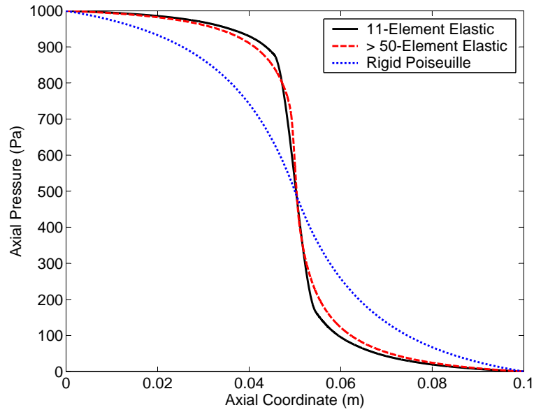
Figure 3. Axial pressure as a function of axial coordinate for a converging-diverging elastic tube with conic geometry having L = 0.1 m, R_{min} = 0.005 m, R_{max} = 0.01 m, and \beta = 236.3 Pa.m. The fluid properties are: \rho = 1000 kg.m -3 and \mu = 0.01 Pa.s while the inlet and outlet pressures are: p_i = 1000 Pa and p_o = 0.0 Pa. The Poiseuille-type flow uses a rigid tube with the same unstressed geometry and the same \mu and boundary pressures. The converged flow rate for the elastic Navier-Stokes and rigid Poiseuille-type flows are respectively: Q_e = 0.000255889 m 3 .s -1 and Q_r = 0.000842805 m 3 .s -1 while the analytic flow rate for the rigid tube as obtained from the first equation in Table 2 is Q_a = 0.000841498 m 3 .s -1 .
