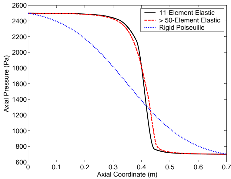
Figure 6. Axial pressure as a function of axial coordinate for a converging-diverging elastic tube with hyperbolic cosine geometry having L = 0.7 m, R_{min} = 0.05 m, R_{max} = 0.08 m, and \beta = 3889.4 Pa.m. The fluid properties are: \rho = 700 kg.m -3 and \mu = 0.0075 Pa.s while the inlet and outlet pressures are: p_i = 2500 Pa and p_o = 700 Pa. The Poiseuille-type flow uses a rigid tube with the same unstressed geometry and the same \mu and boundary pressures. The converged flow rate for the elastic Navier-Stokes and rigid Poiseuille-type flows are respectively: Q_e = 0.0427687 m 3 .s -1 and Q_r = 1.4184 m 3 .s -1 while the analytic flow rate for the rigid tube as obtained from the fourth equation in Table 2 is Q_a = 1.416296 m 3 .s -1 .
