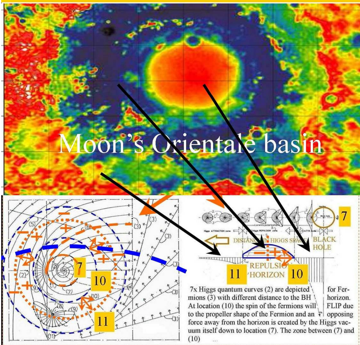
Figure 2, Mare Orientale, with cross section through the multiple new physics black hole boundaries.
