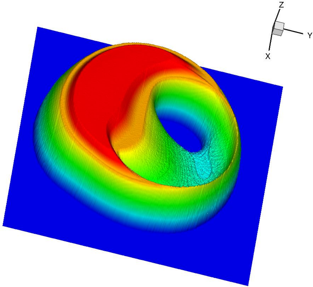
Figure 4 – Isometric pseudo-3D reconstruction of Figure 3 in order to better see the main properties of the surroundings of the event horizon of black hole Sgr A*.
