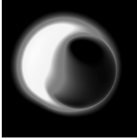
Figure 3 – BW version of the image simulation of Figure 2.
