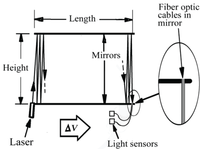
Figure 2. Calkins' Generic Experimental Apparatus
