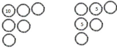
SPIN COUNT DECREASED BUT THE NUMBER OF PARTICLE SPINNING INCREASED
