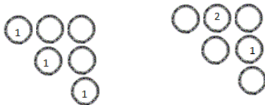
PARTICLE GAINING SPIN COUNT
