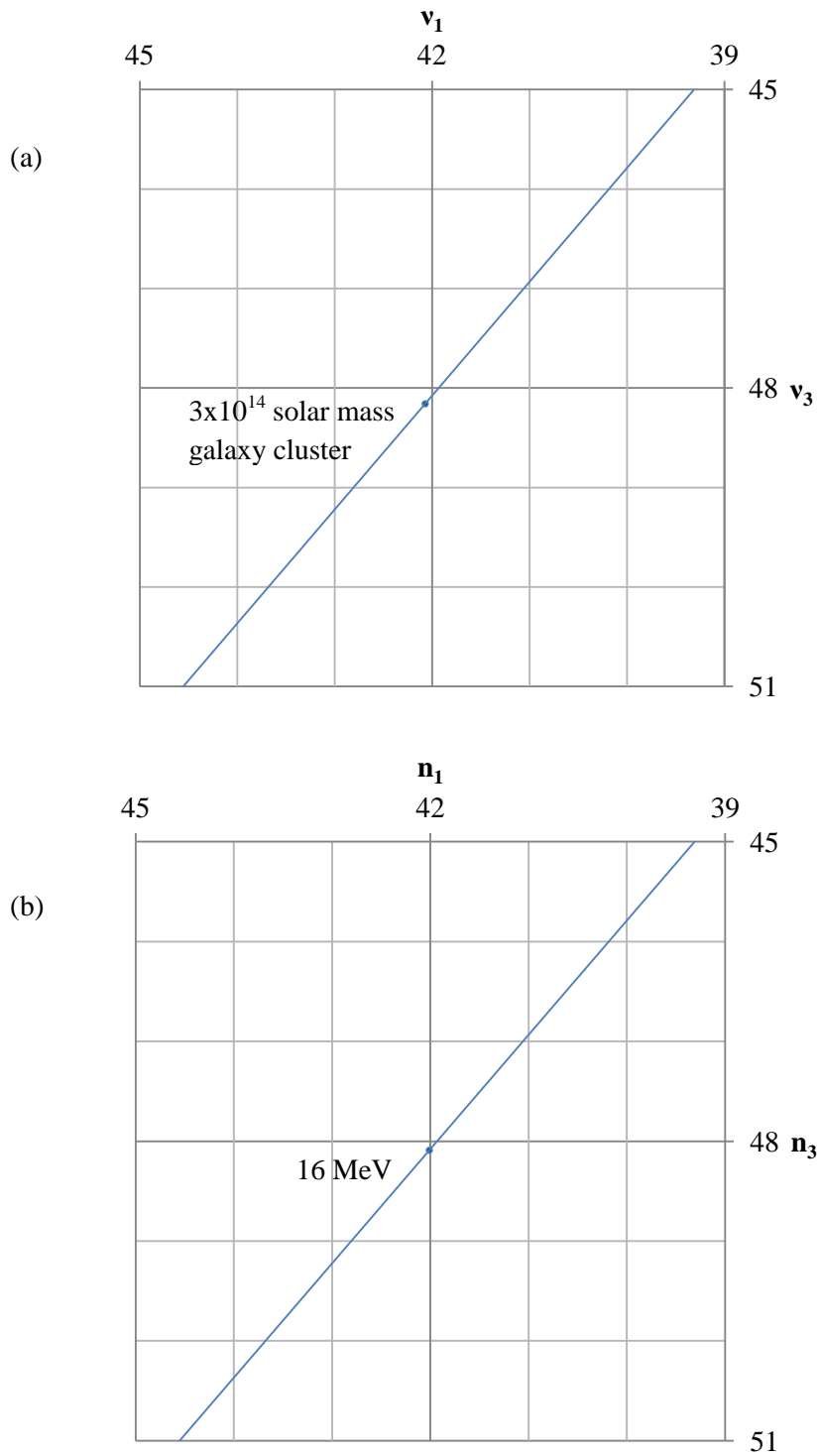
Figure 4: (a) The length scale corresponding to the mass, 3 \times 10^{14} solar masses, of a typical galaxy cluster, on the trans-Planckian levels of Sequences 1 and 3. (b) The mass scale, 16 MeV, associated with the proposed dark matter particles of mass 7.1 keV and 35 GeV, on the levels of Sequences 1 and 3.
