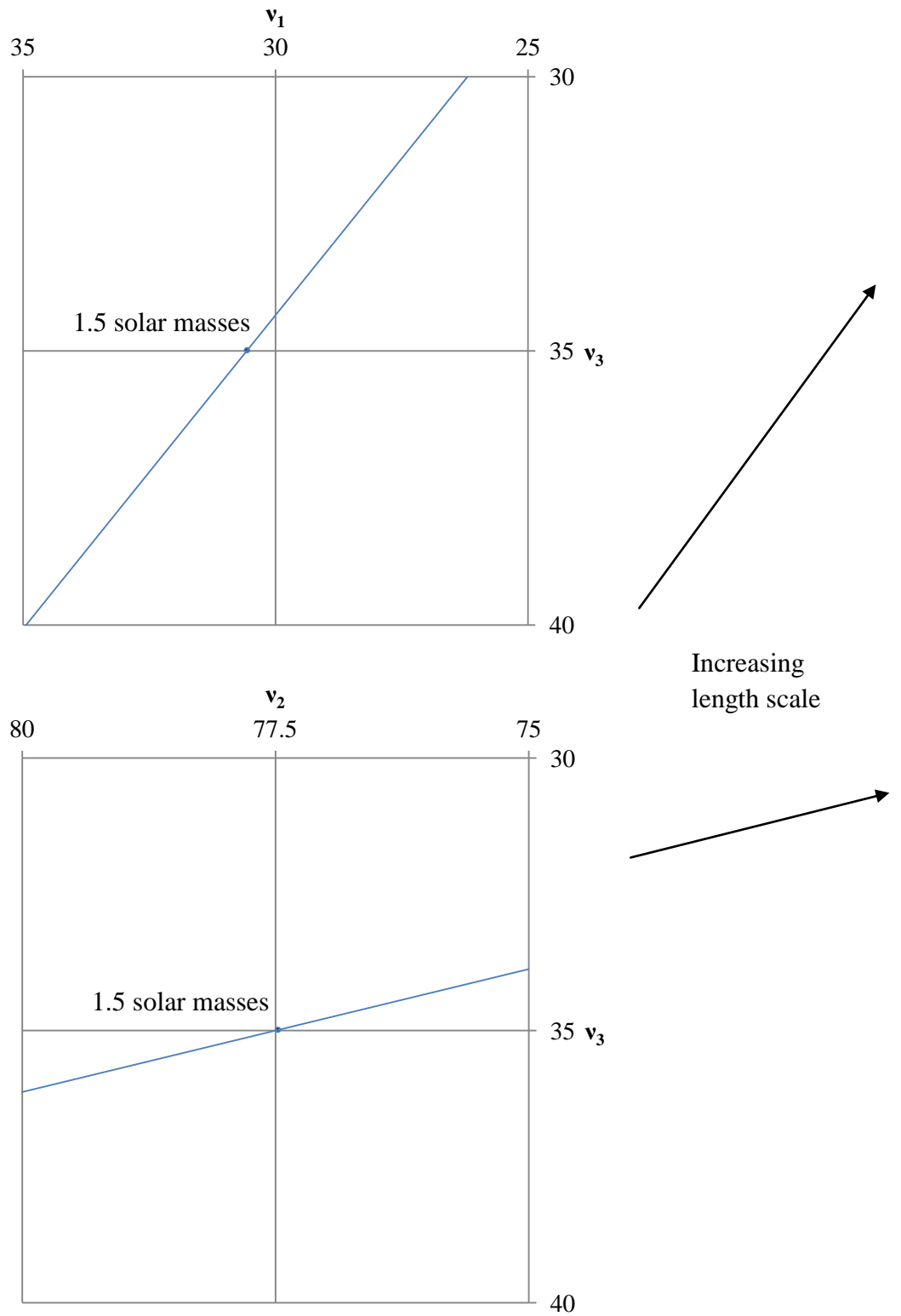
Figure 1: The length scale corresponding to a TOV limit of 1.5 solar masses on the trans-Planckian levels of Sequences 1, 2 and 3. Scales are constrained to lie on a straight line (shown here in blue) since level numbers in the three Planck sequences are in constant ratio.
