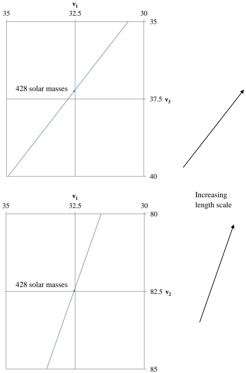
Figure 2: The length scale corresponding to the mass (428 solar masses) of the intermediate-mass black hole in M82 X-1, on the trans-Planckian levels of Sequences 1, 2 and 3.
