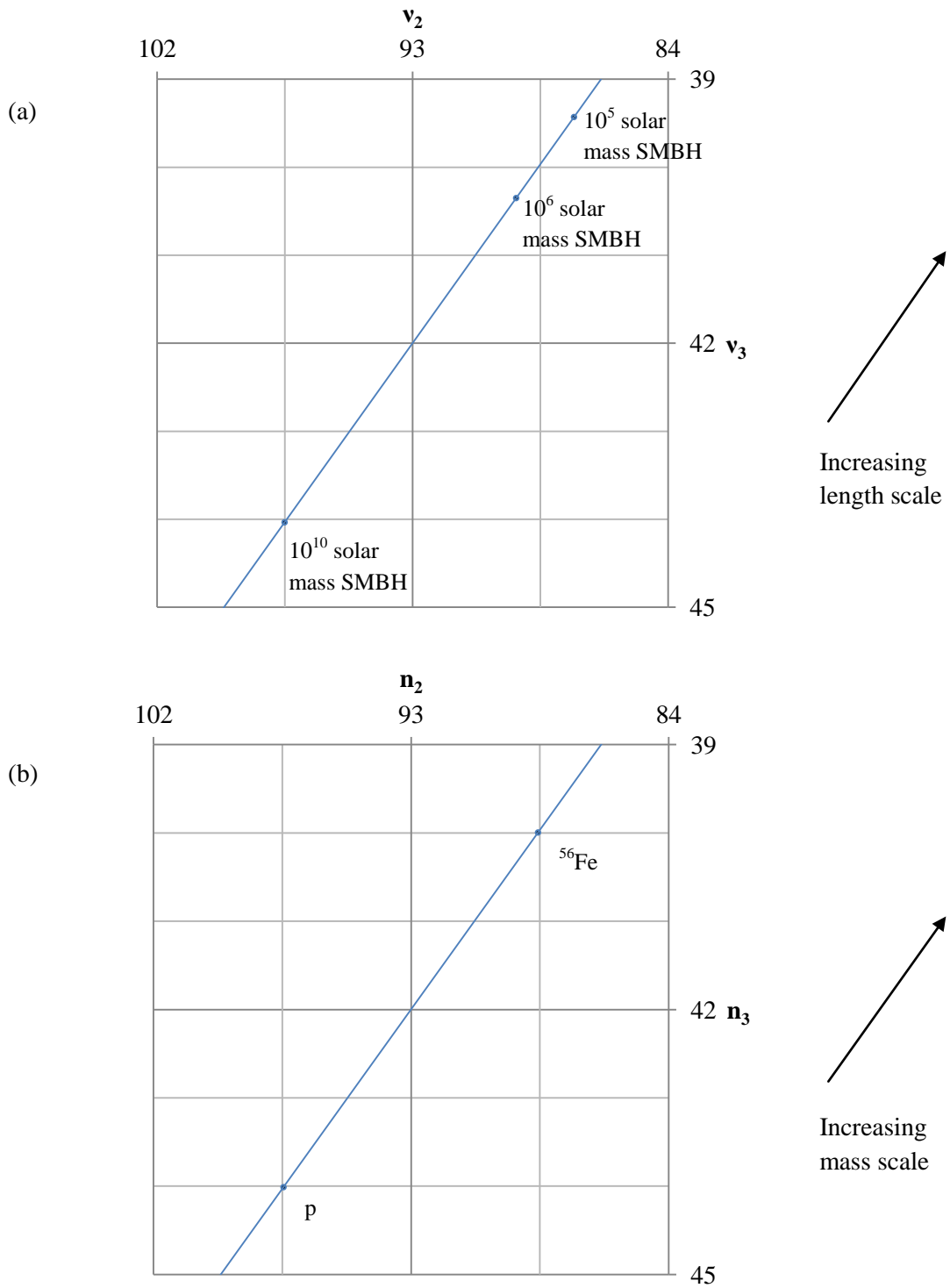
Figure 3: (a) Supermassive black holes on levels of trans-Planckian length scale in Sequences 2 and 3. The distribution of SMBH length scales is centred on (93, 42). (b) The proton and the ^{56}\text{Fe} nucleus arranged symmetrically about (93, 42) on the mass levels of Sequences 2 and 3.
