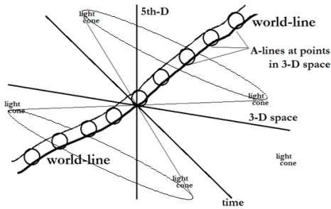
The world-line of an event in the light cone of 4-D space-time is an infinitesimally miniscule cylinder in the 5th-D of space-time
