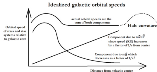
The halo is like a shadow or mirror image of the core curvature due to the centrifugal force (equal and opposite) of gravity due to the rest of the universe represented by \Gamma
