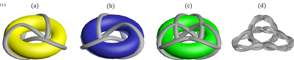
Figure 5: The (a) left-handed trefoil - (3,2) torus knot - laying on the left Clifford torus C_{-1} and (b) the right-handed trefoil laying on the, mirrored, right Clifford torus C_1 , are merged into one (c) third middle Clifford torus C_0 that (d) further compresses and finally disappears. What is left is a closed left+right handed trefoil knot loop.
