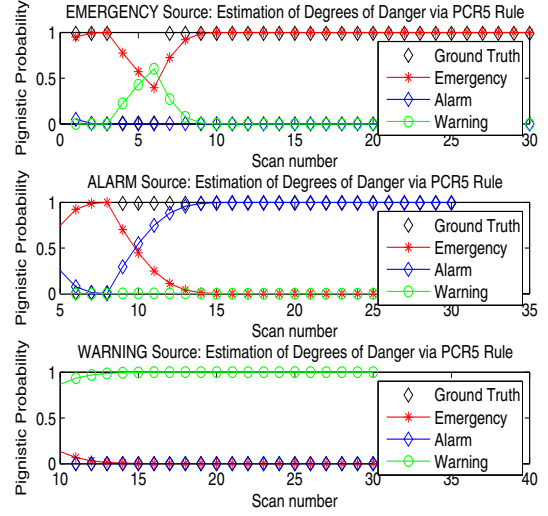
Fig. 2. PCR5 rule Performance for danger level estimation.
