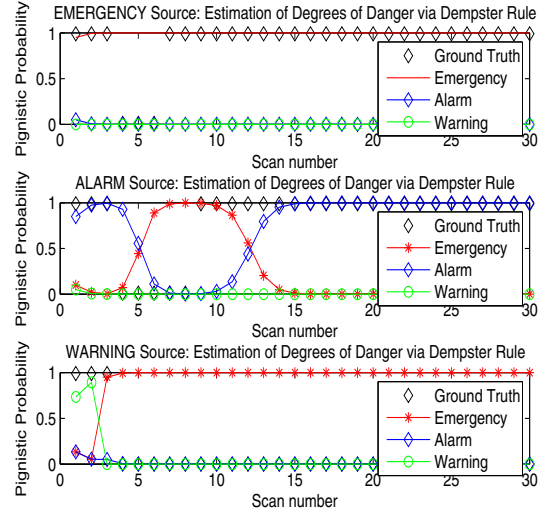
Fig. 3. Dempster's rule Performance for danger level estimation.
