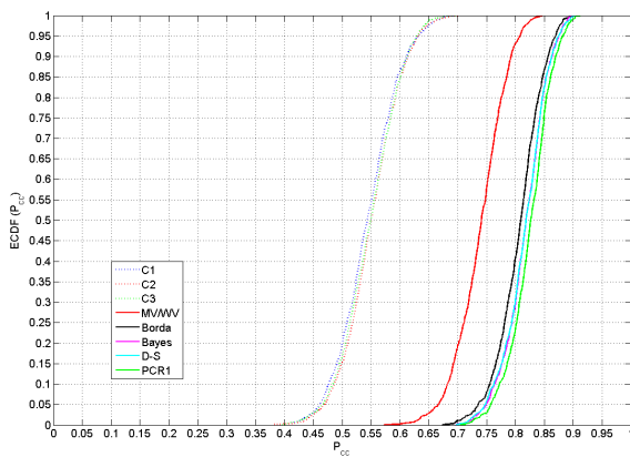
Fig. 2. ECDF versus P_{cc} with complementary confusion matrices (estimation from 30 samples per class).
