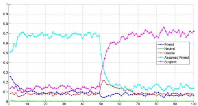
Figure 9. DS m result after 100 Monte-Carlo runs.
