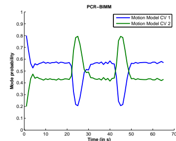
Figure 5: Motion Model Probability of the PCR-BIMM
