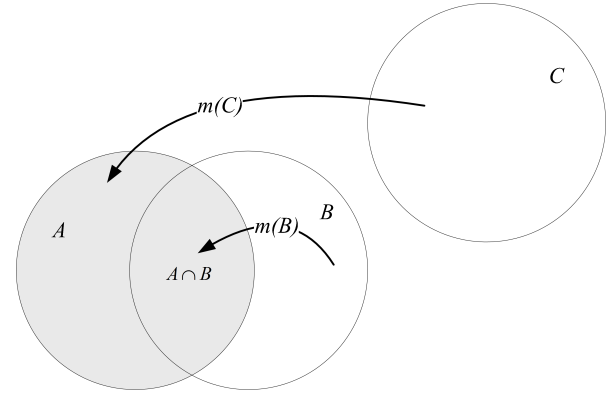
Figure 1. Mass transfer in case of application of the rule (4)
