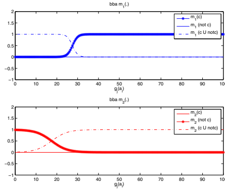
Fig. 3 Bba's m_1(.) and m_2(.) to combine.
