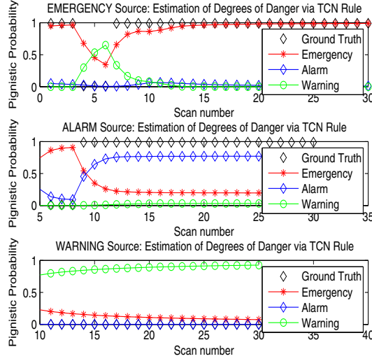
Fig. 1. TCN rule Performance for danger level estimation.
