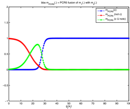
Fig. 4 m_{ih}^j(.) obtained from the PCR5 fusion of m_1(.) with m_2(.) .
