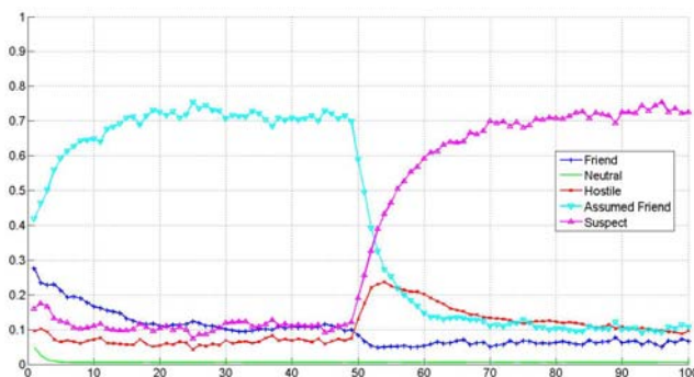
Figure 12: DSmt result after 100 runs and input filter.
