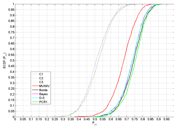
Fig. 3. ECDF versus P_{cc} with complementary confusion matrices (estimation from 10 samples per class).
