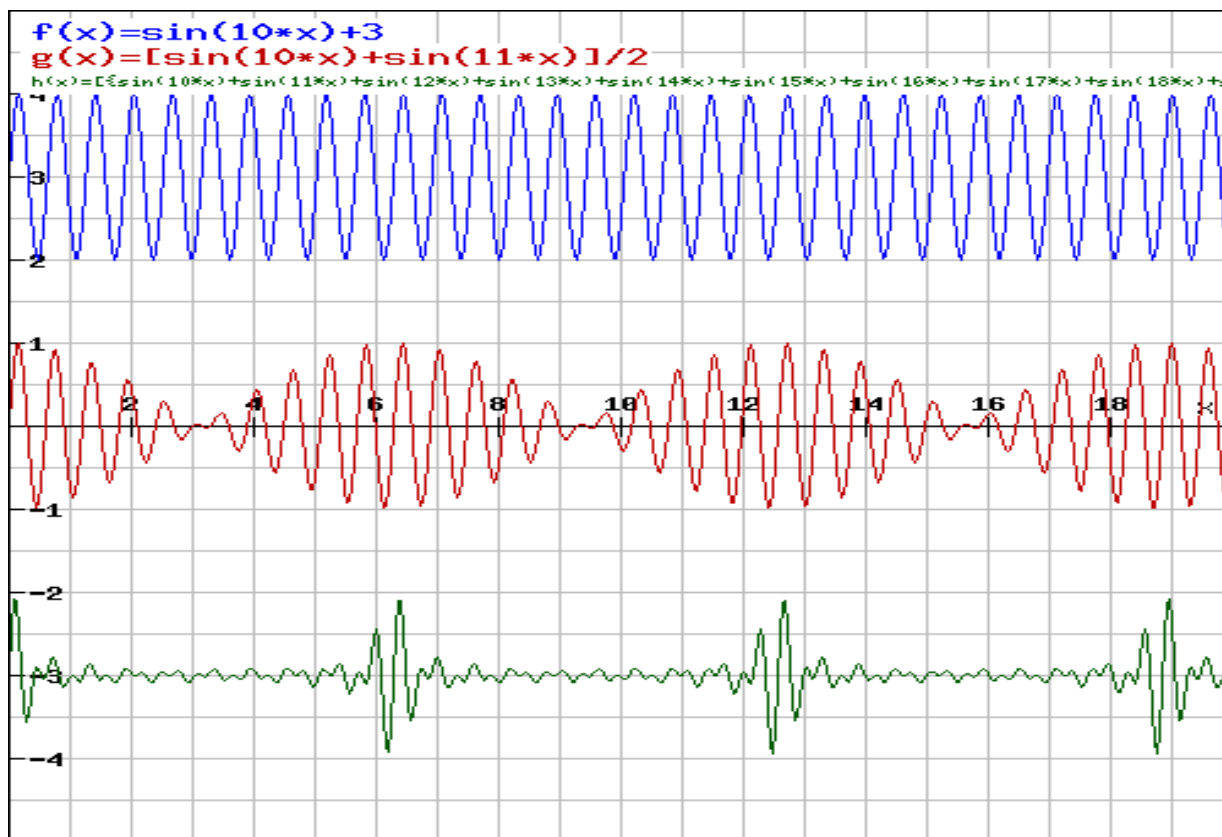
Fig.1: (i) Blue curve, on the top, shows a wave of purely single frequency, \sin(10*x) ; (ii) the red curve, in the middle, shows that when two waves get added, their amplitude start varying in space and time; and (iii) the green curve, at the bottom, shows that when so many waves of
