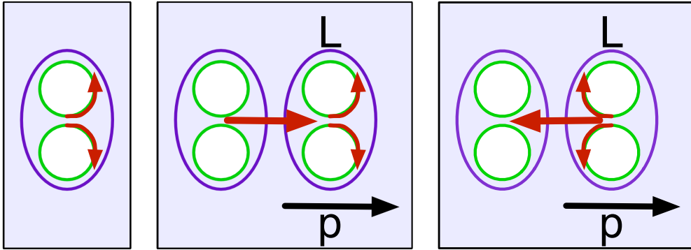
FIG. 1: The diagrams show constant \phi slices of S^1 \times P^2 . The red arrows are \partial^\mu y . The left diagram shows \partial^\mu y on a S^1 \times P^2 , in the +\theta direction. The other two diagrams show a lepton L becoming a neutrino. The lepton transfers charge to another S^1 \times P^2 . The transfer of charge gives L momentum p in the opposite direction. Gravity produces a background rotation, with \partial^\mu y = \partial^\mu(k_\nu A^\nu) . Because of the charges on each S^1 \times P^2 , \partial^\mu(k_\nu A^\nu) points either towards L (on the left) or away from L (on the right). The vector field \partial^\mu y must be consistent, therefore \partial^\mu(k_\nu A^\nu) must match the +\theta or -\theta arrows on L . The sign of the charge determines \partial^\mu(k_\nu A^\nu) . Therefore the relation between quantum phase \theta and the linear momentum p for neutrinos is opposite to that of antineutrinos. Beginning with a neutrino L and producing a charged lepton would reverse the direction of p in the diagram.
