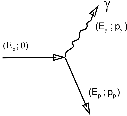
Figure 28: Feynman diagram
