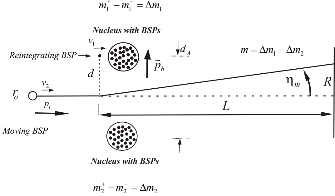
Figure 14: Bending of BSPs
