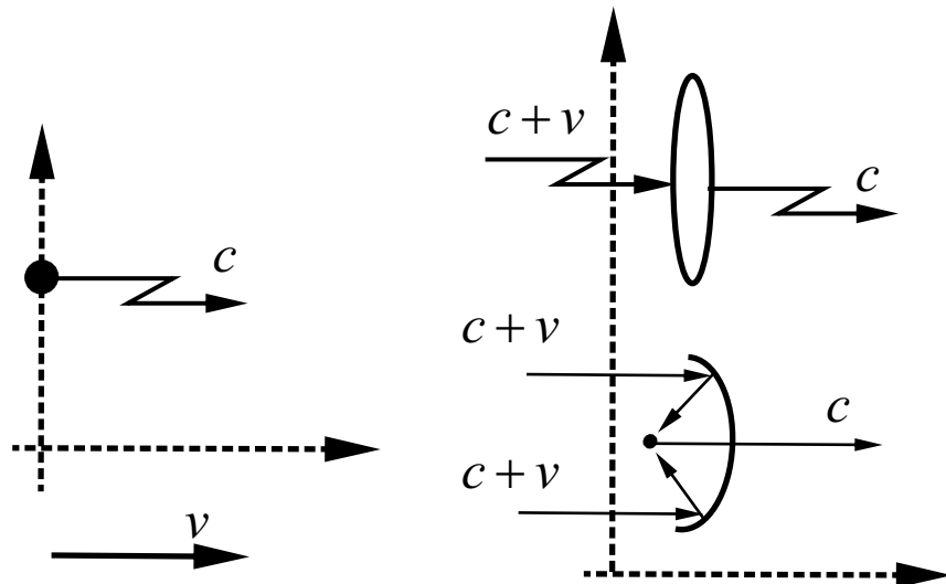
Figure 31: Light on relative moving receivers
