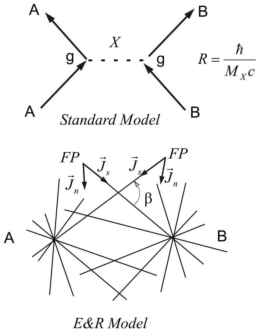
Figure 11: Differences between the Standard and the E & R Models
