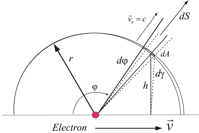
Figure 21: Emitted Energy flux density dS of a moving electron
