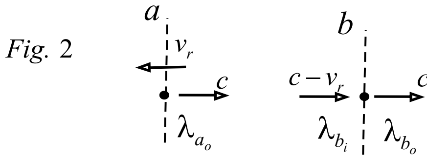
Figure 34: Sagnac experiment
