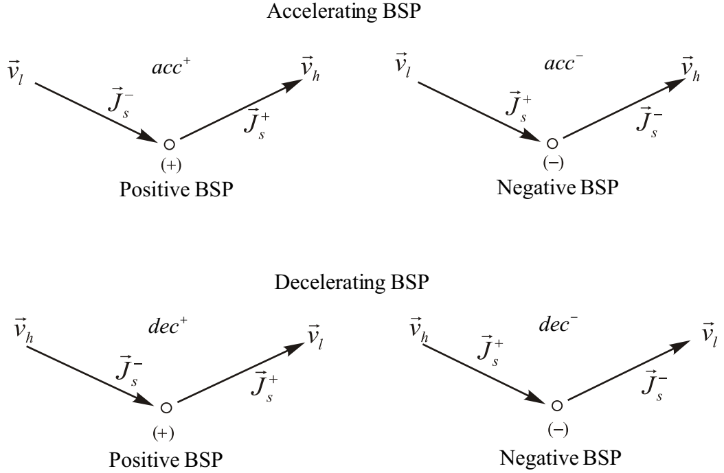
Figure 24: Conventions for BSPs
