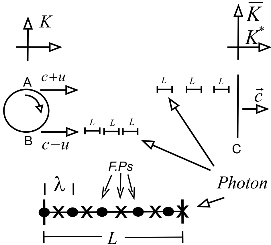
Figure 29: Emission Theory.
