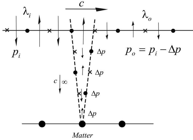
Figure 37: Loss of energy of a BSP with v = c
