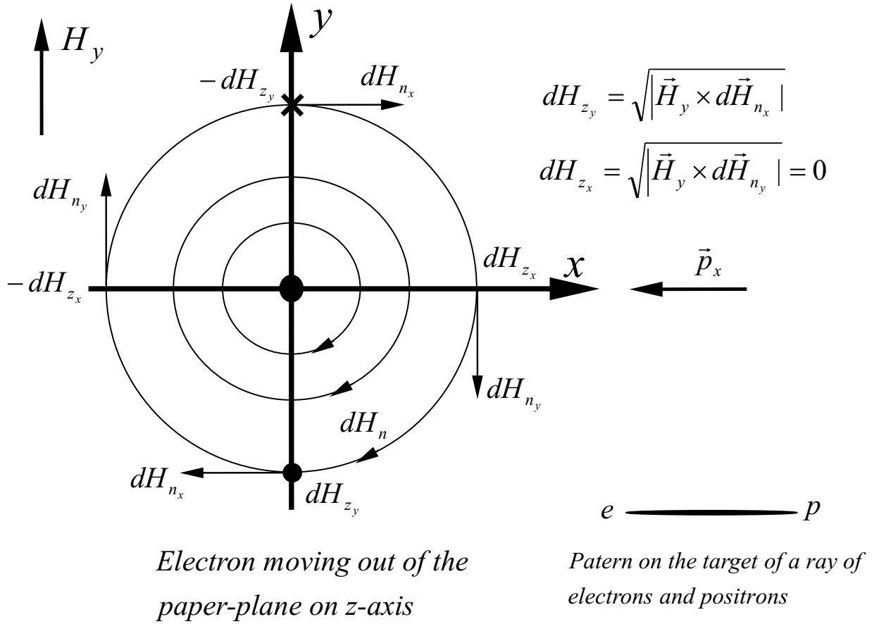
Figure 12: Stern-Gerlach-experiment with an homogeneous magnetic field
