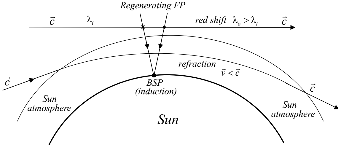
Figure 38: Refraction and red-shift at the Sun
