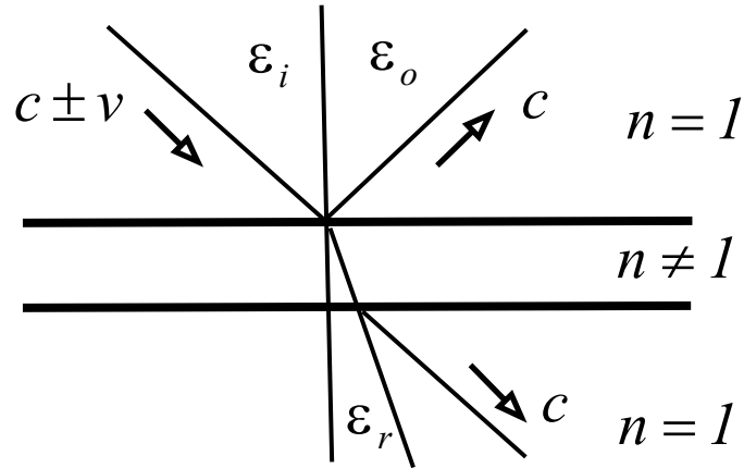
Figure 30: Light speed at reflections and refractions
