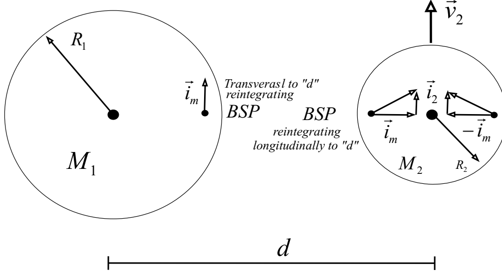
Figure 18: Ampere gravitation
