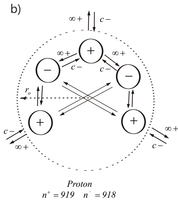
Figure 25: Neutron and proton composed of accelerating positrons and decelerating electrons
