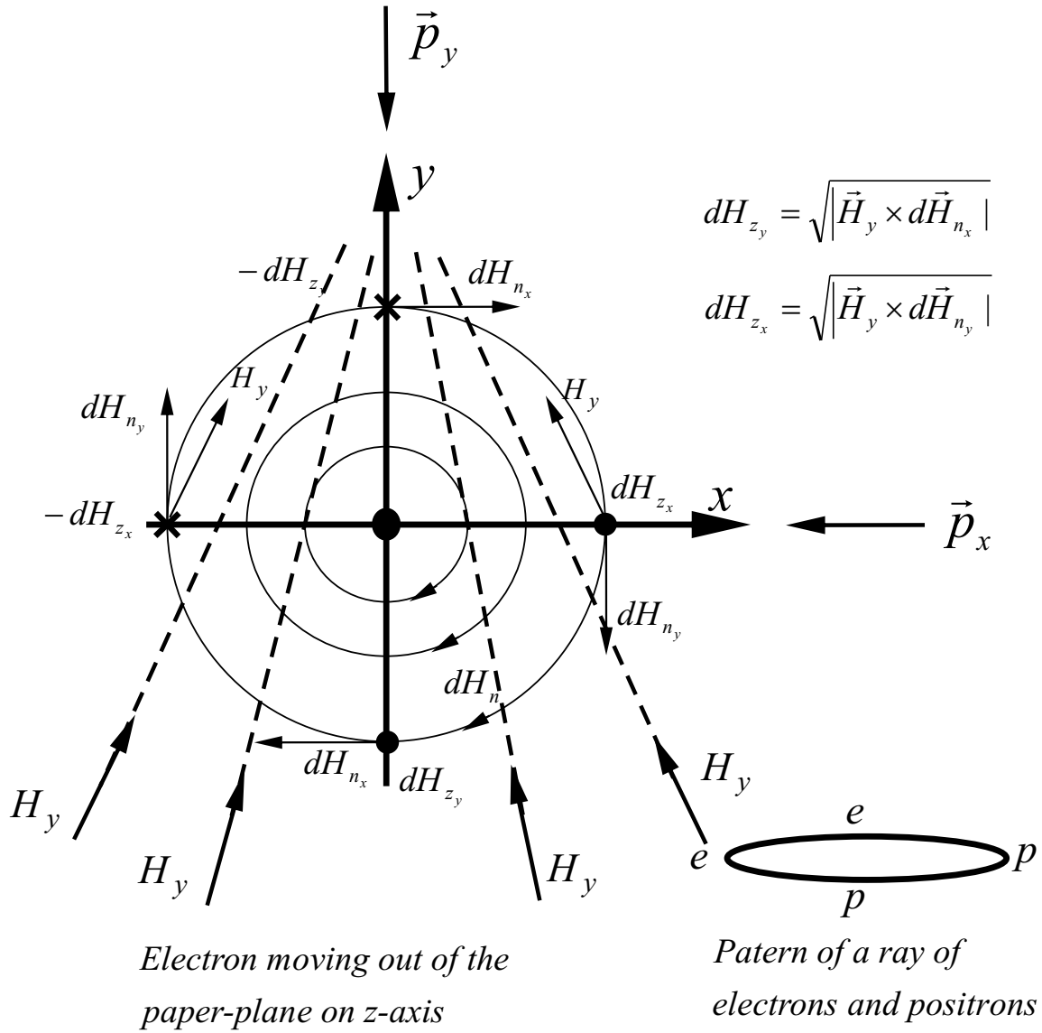
Figure 13: Stern-Gerlach-experiment with an inhomogeneous magnetic field
