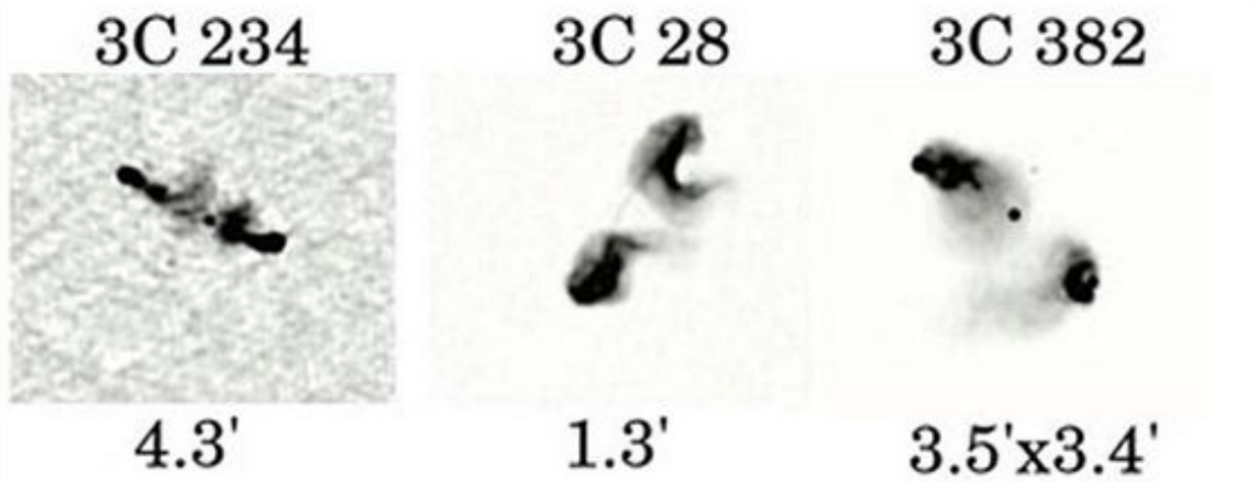
Figure 11, Several examples of pairing and splitting black hole with the principle mechanisms at the top of the image.
