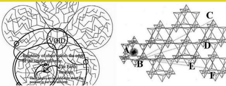
Figure 8, with the Higgs oscillating truncated tetrahedron vacuum lattice.
